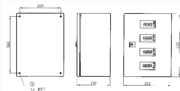
Wall mounting housing WAG 03/04 for up to 4 DA 10/12/14
