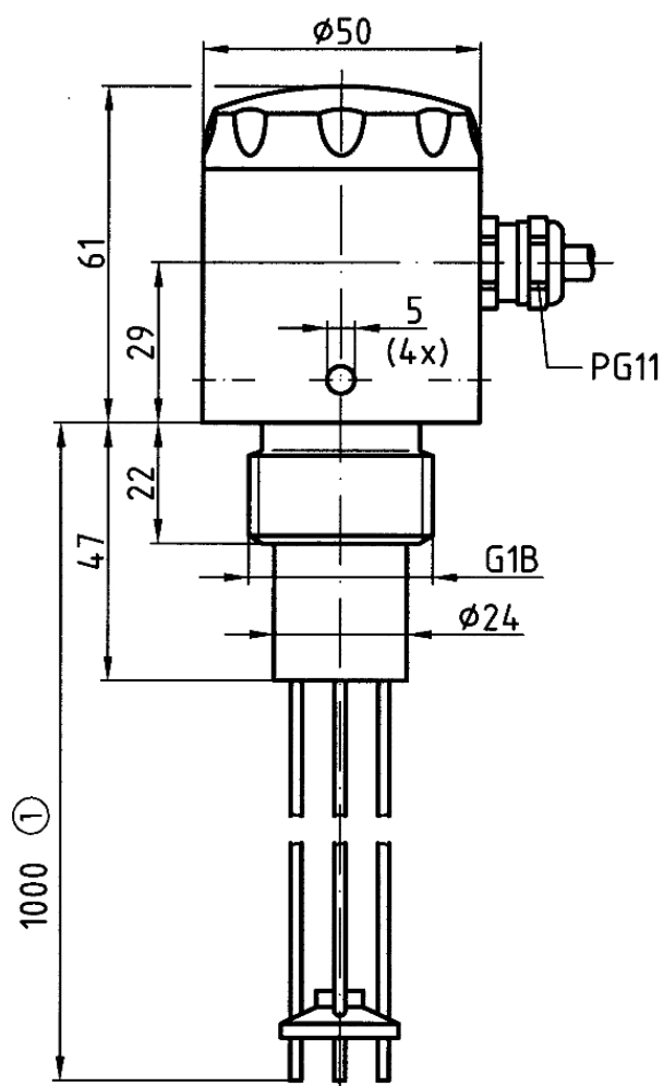
Triple-rod probe LSM 01
