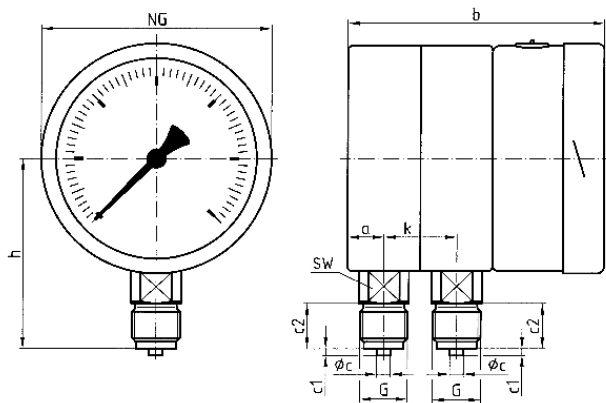
Bottom connection
