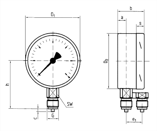
NG 100/160 – bottom connection
