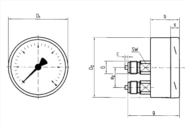
Dimensions (mm)
