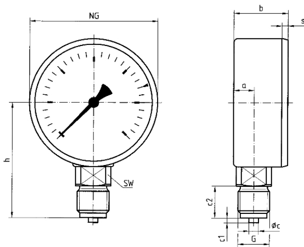
Dimensions (mm)
