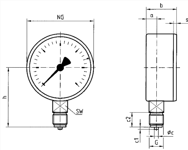
Dimensions (mm)
