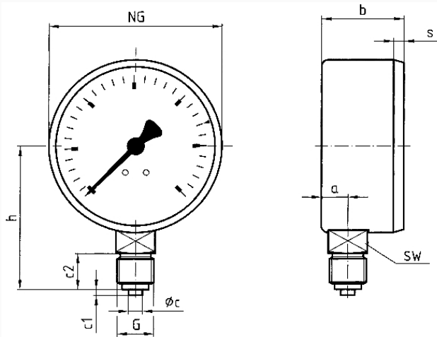
Dimensions (mm)
