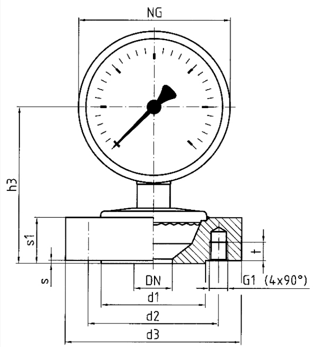
Dimensions (mm)
