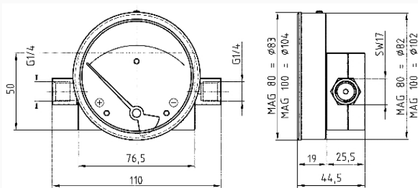
Dimensions (mm)
