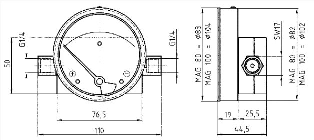
Dimensions (mm)
