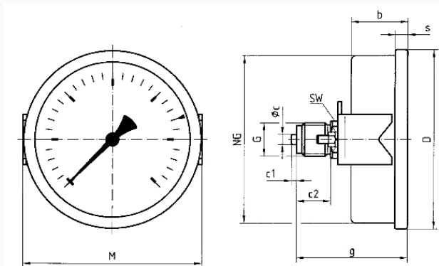
NG 100 – centre back connection, with clamp fixing
