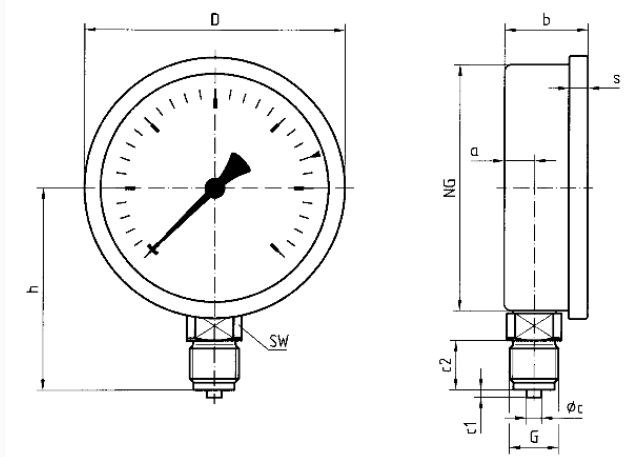
Dimensions (mm)
