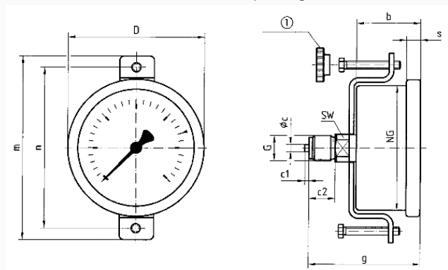
Centre back connection, with clamp fixing
