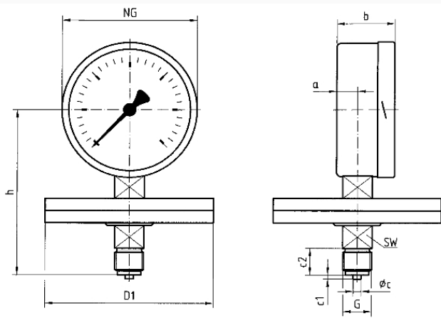
bottom connection, measuring flange ø 160
