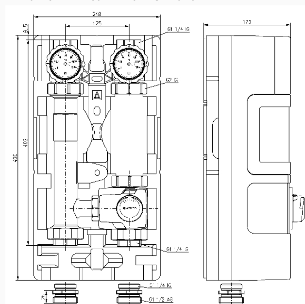
Dimensions (mm)
