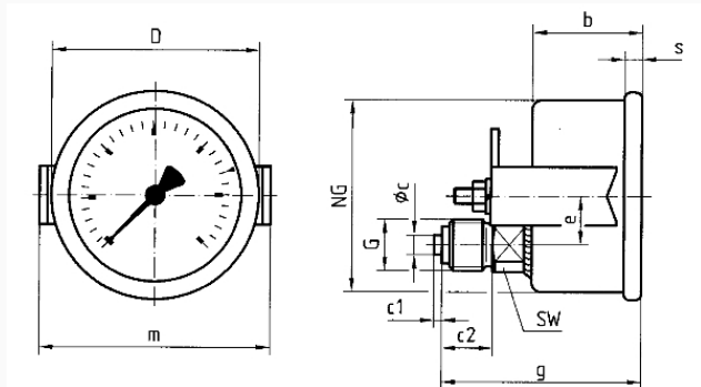
NG 50 – bottom back connection, with clamp fixing
